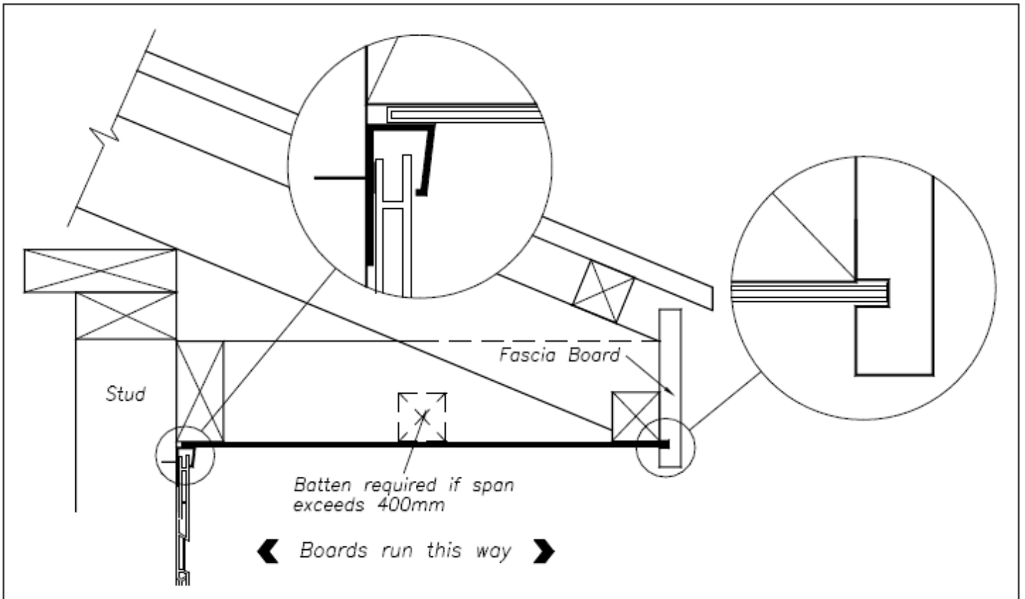
Fig 21 Soffit Detail
