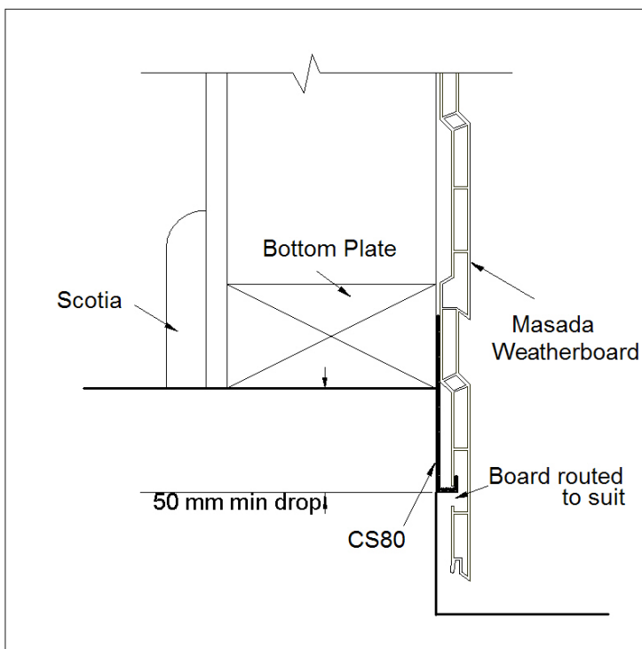
Fig 2 Half Drop Starting
