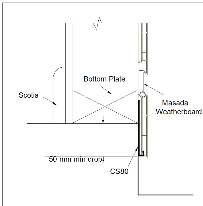
Fig 1 Bottom Wall Starter
