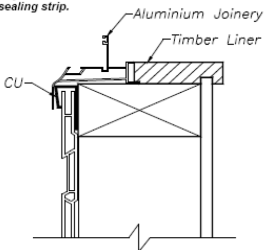
Fig 7 Sill
