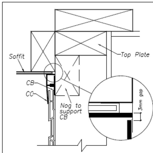
Fig 16a Top Wall—Under Eave CB/CC
