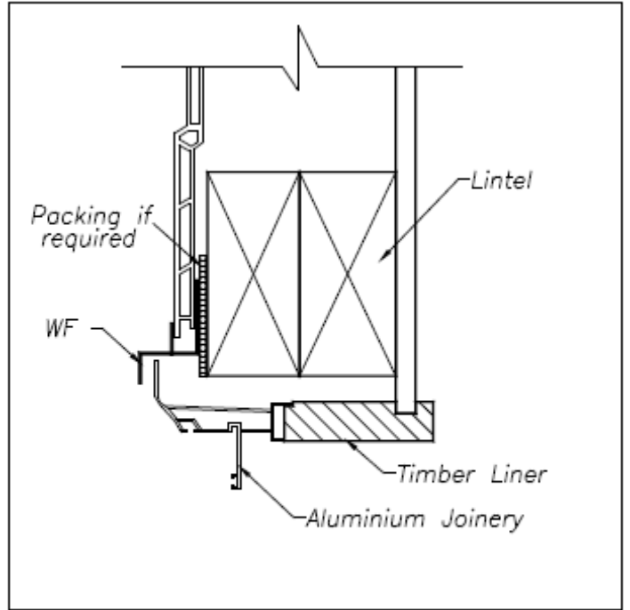
Fig 13 Window Head
