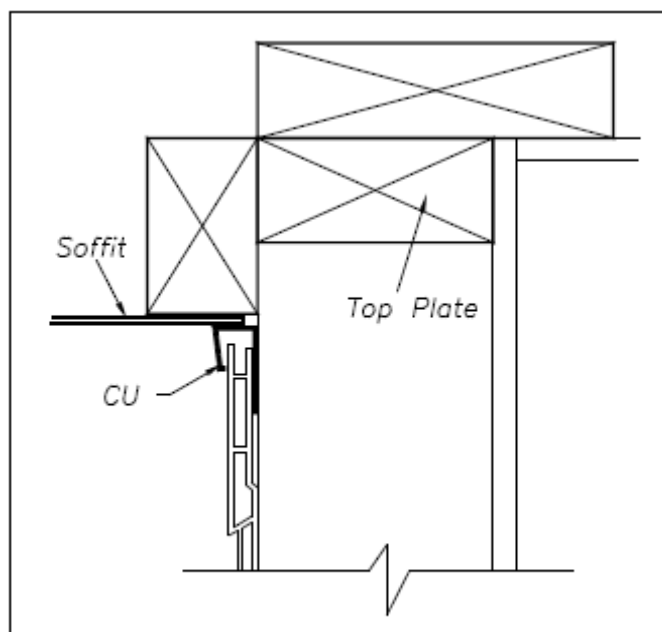
Fig 16b Alternative CU Under Eave
