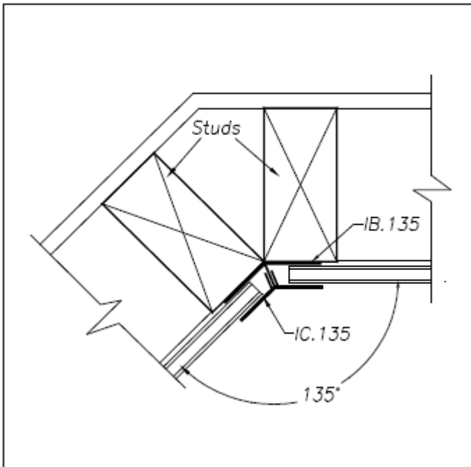
Fig 5 135° Internal Corner
