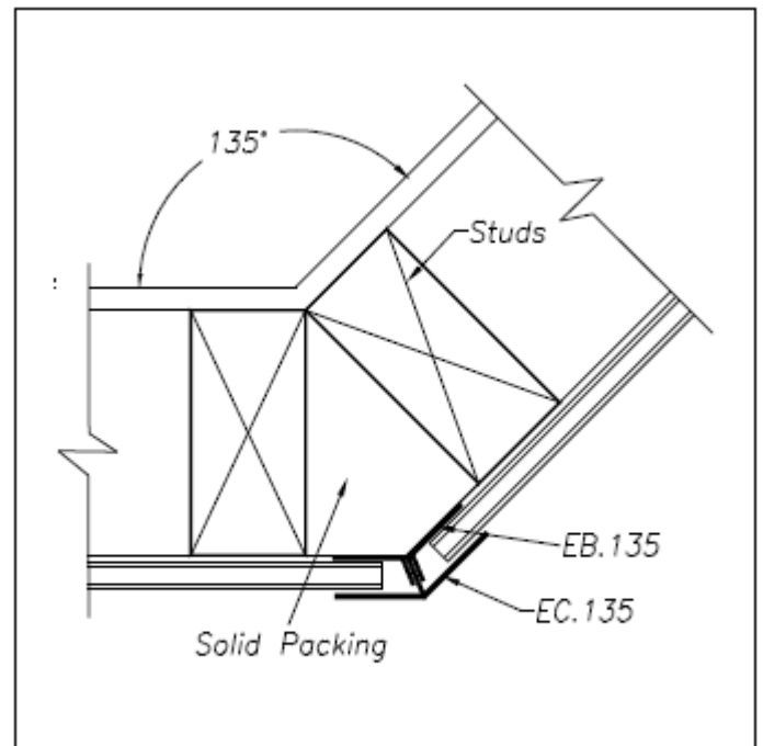
Fig 6 135° External Corner
