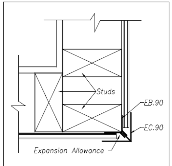
Fig 4 90° External Corner
