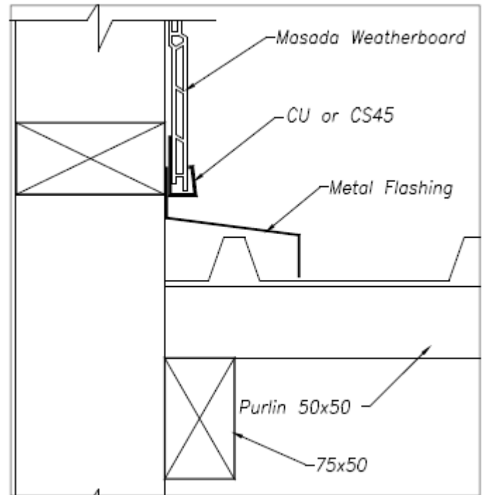
Fig 18 Roof Flashing
