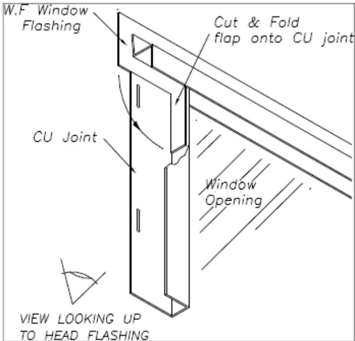
Fig 12 Head Flashing
